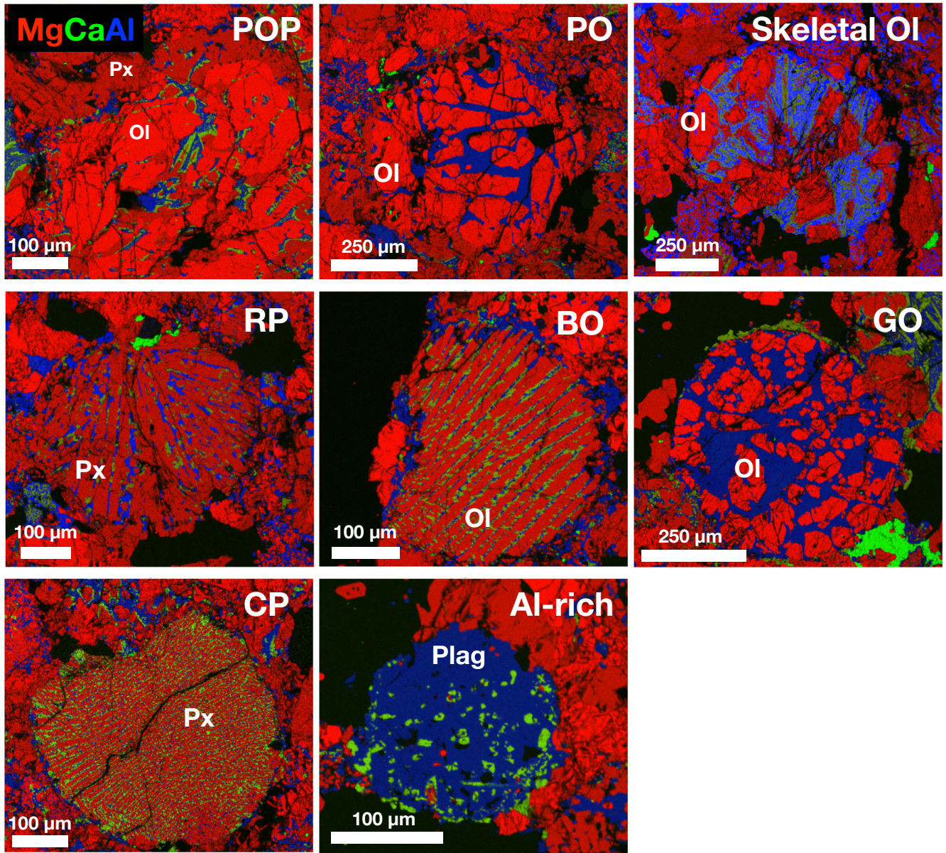
Fig. 7. Composite RGB EDS maps of different types of chondrules found in the Hamburg type specimen section. Abbreviations: POP = porphyritic olivine with pyroxene; porphyritic olivine (PO), Ol = olivine; Px = pyroxene; radial pyroxene (RP); barred olivine (BO); cryptocrystalline (C) chondrules with pyroxene, granular olivine (GO). Red = Mg; green = Ca; blue = Al.
