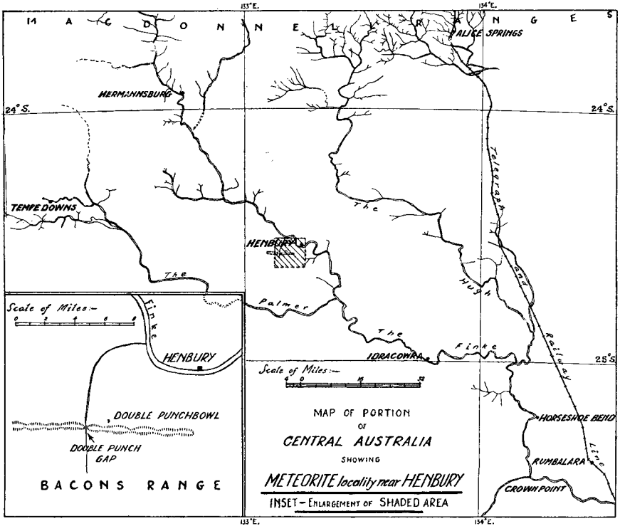
FIG. 1. Sketch-map of the locality.
