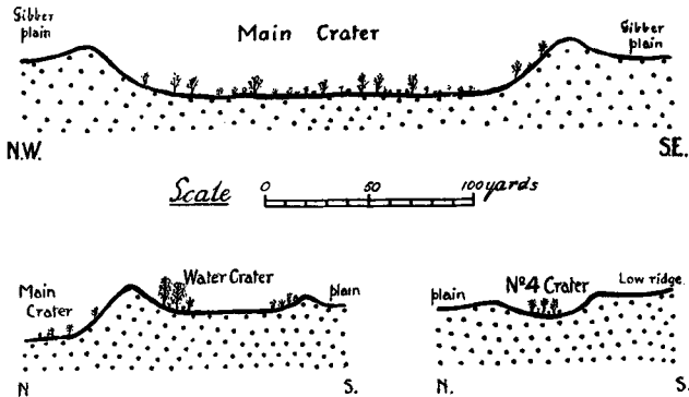
FIG. 3. Sections through the craters.
